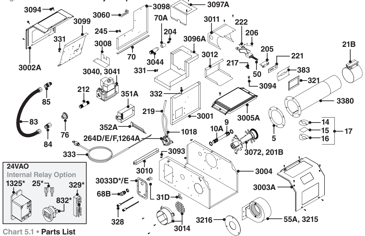
Figure 5.1 • Burner Assembly Components
